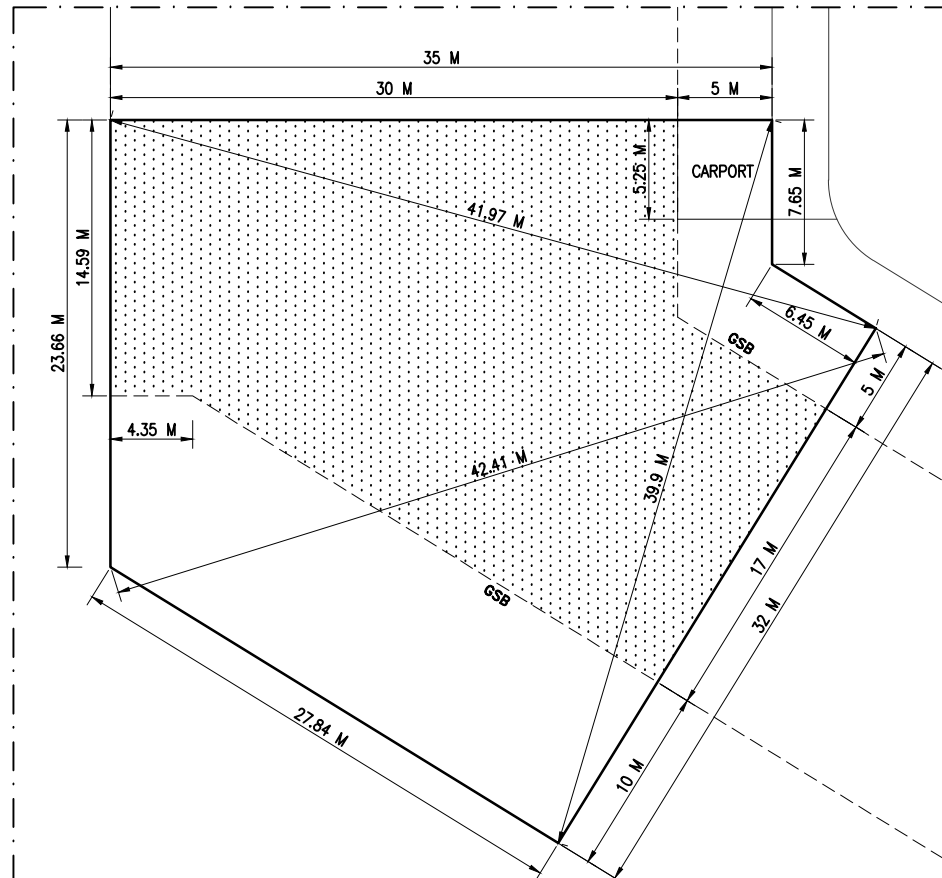
DENAH KAVLING JL.RATNAMAHA NO.17 SKALA 1 : 400
